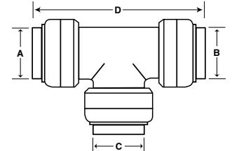
Tee Dimensions
