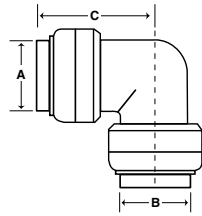
Elbow Dimensions
